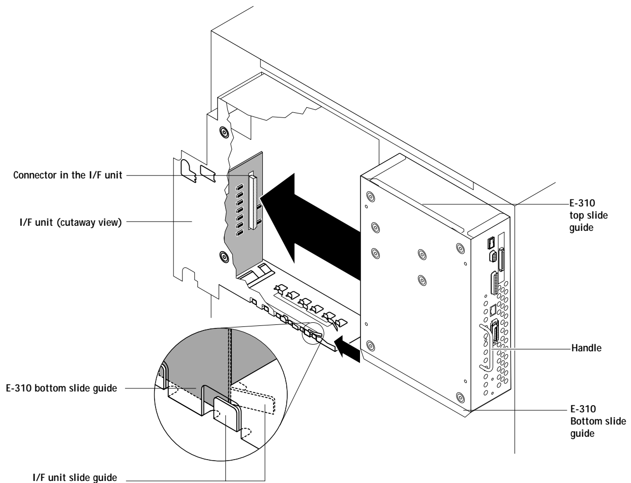
FIGURE 2-4 Installing the E-310 in the I/F unit
